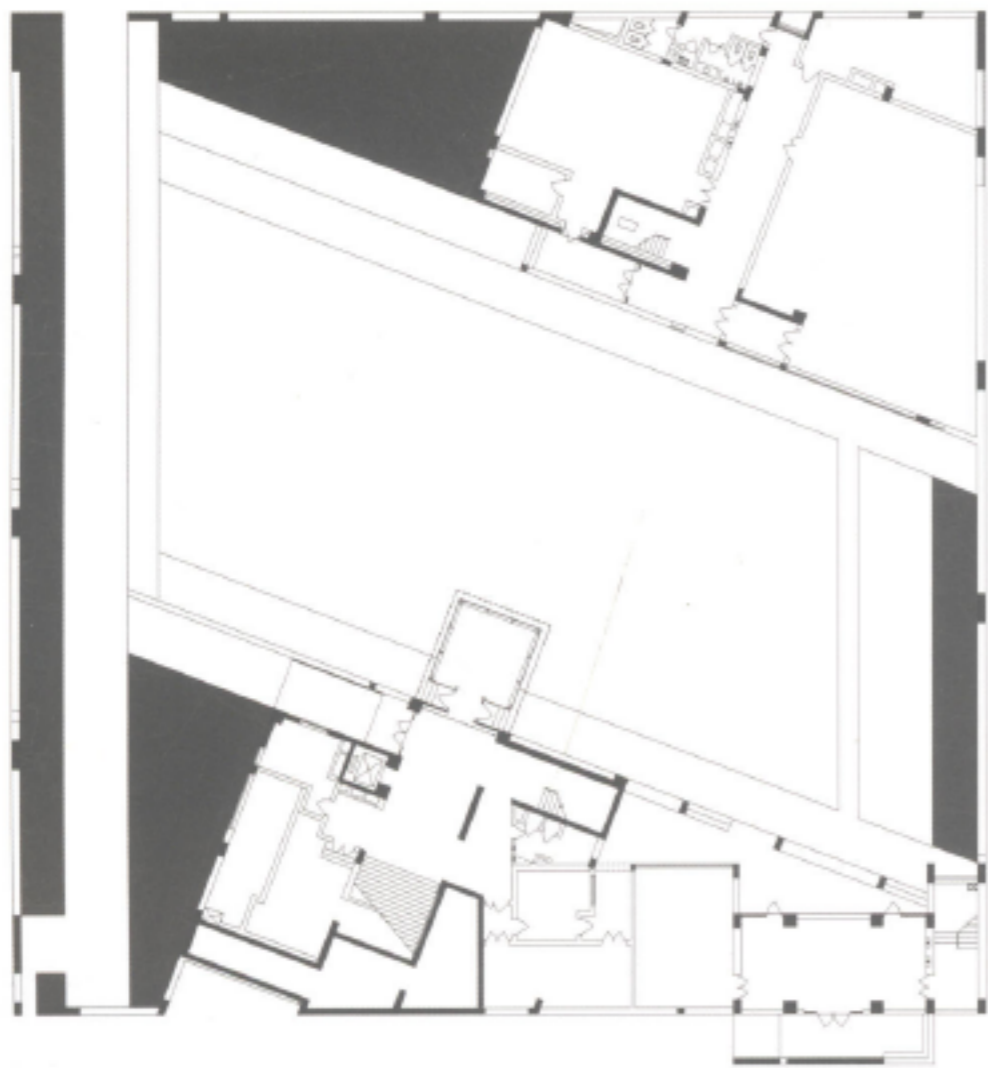
1st floor plan 一層平面圖
