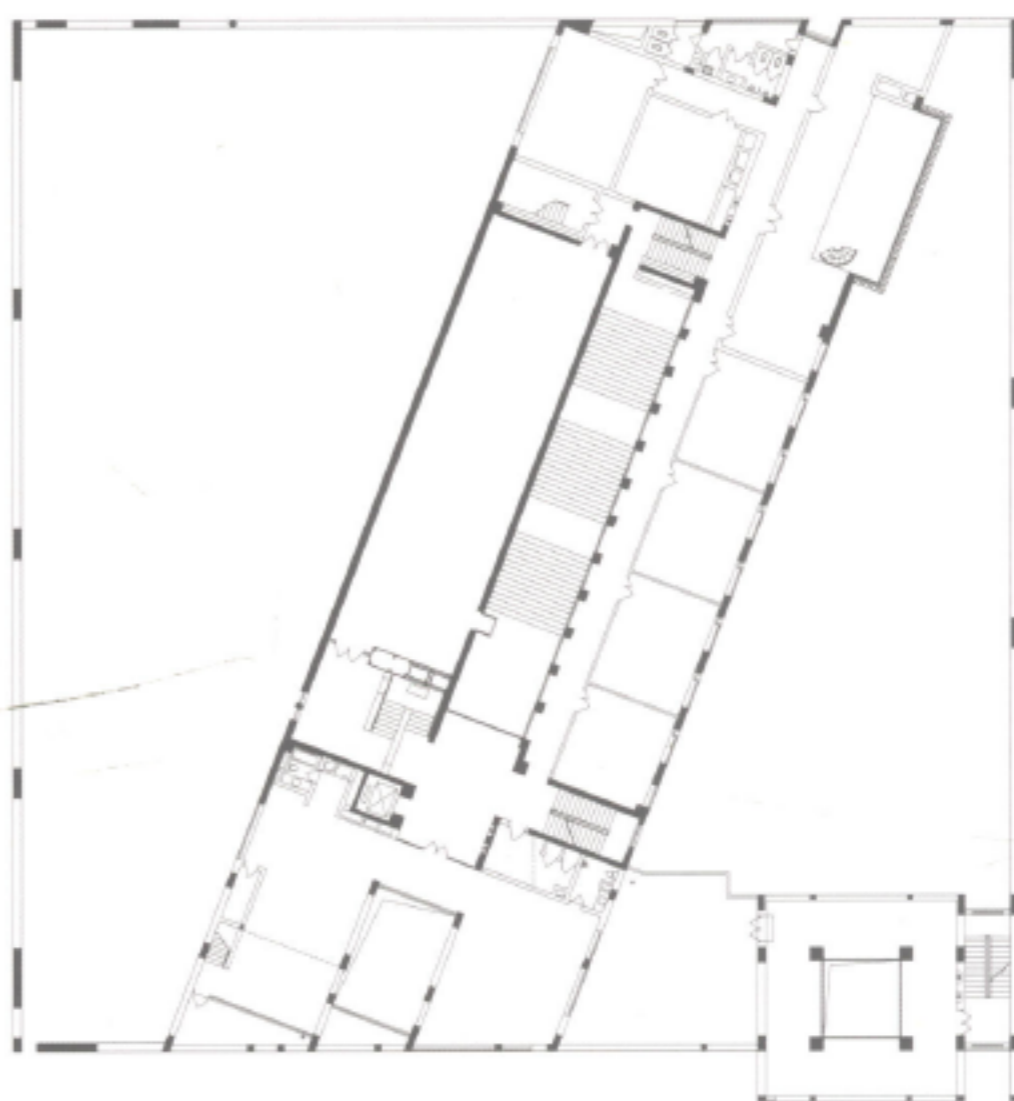
3rd floor plan 三層平面圖
